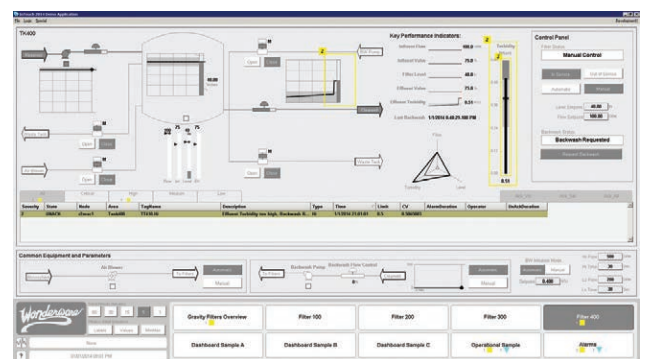
Figure 7 - Level 2 Window Example
