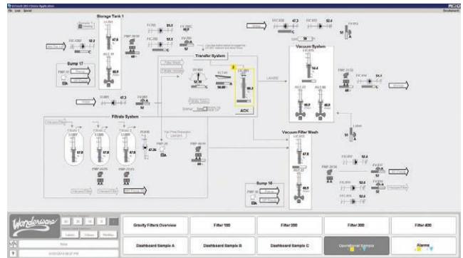
Figure 8 - Level 3 Window Example
